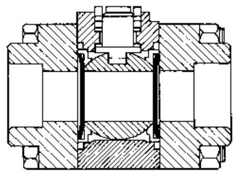
Ball valve
