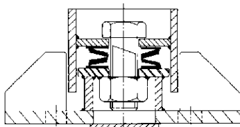
Shock absorption
