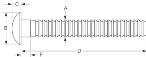
RIVET HEAD
