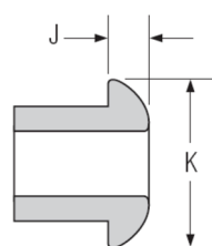
COLLAR - CLEARANCE
