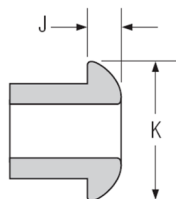
COLLAR - SHORT GRIP CLEARANCE
