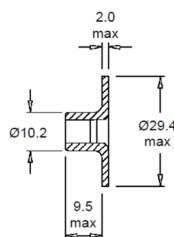
COLLAR - FLAT SLEEVE
