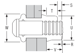
AFTER INSTALLATION
